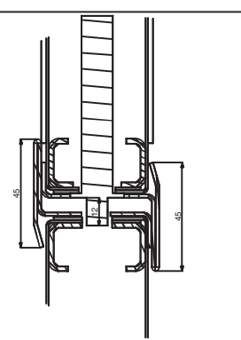
DETAIL 1 SCALE 1:2
