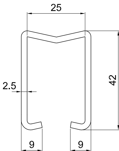
LATERAL VIEW scale 1:1
