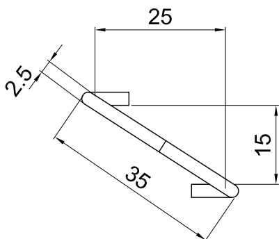
PLAN VIEW scale 1:1
