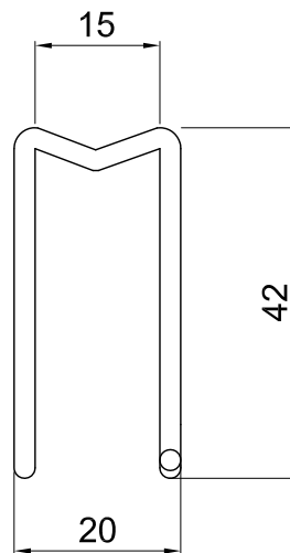
LATERAL VIEW scale 1:1
