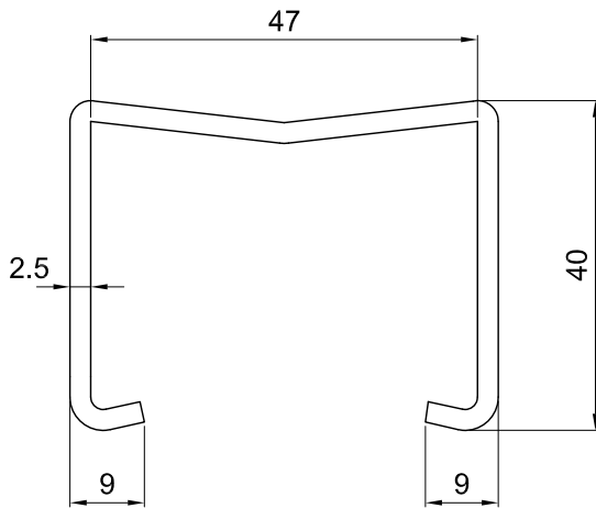
LATERAL VIEW scale 1:1
