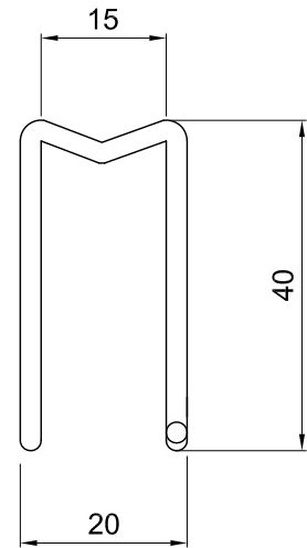
LATERAL VIEW scale 1:1
