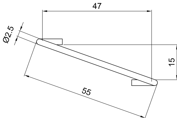
PLAN VIEW scale 1:1
