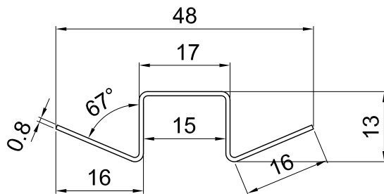
LATERAL VIEW
