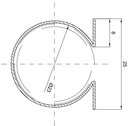
PROFILE SECTION
