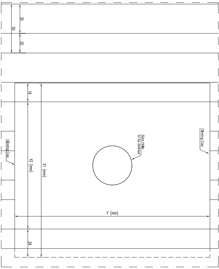
DETAIL 1 - LIGHT BOX scale 1:2
