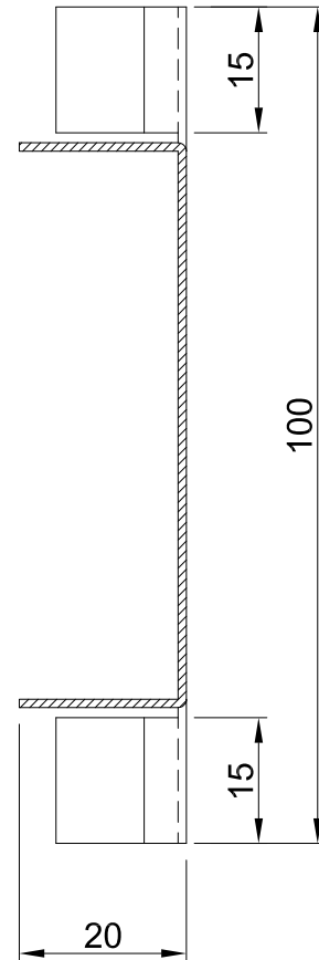
B-B SECTION
