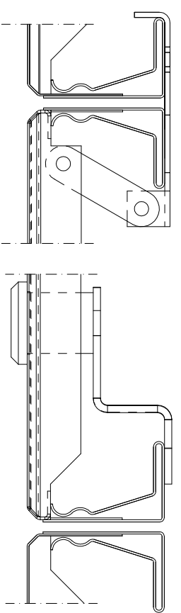
DETAIL 1 scale 1:1
