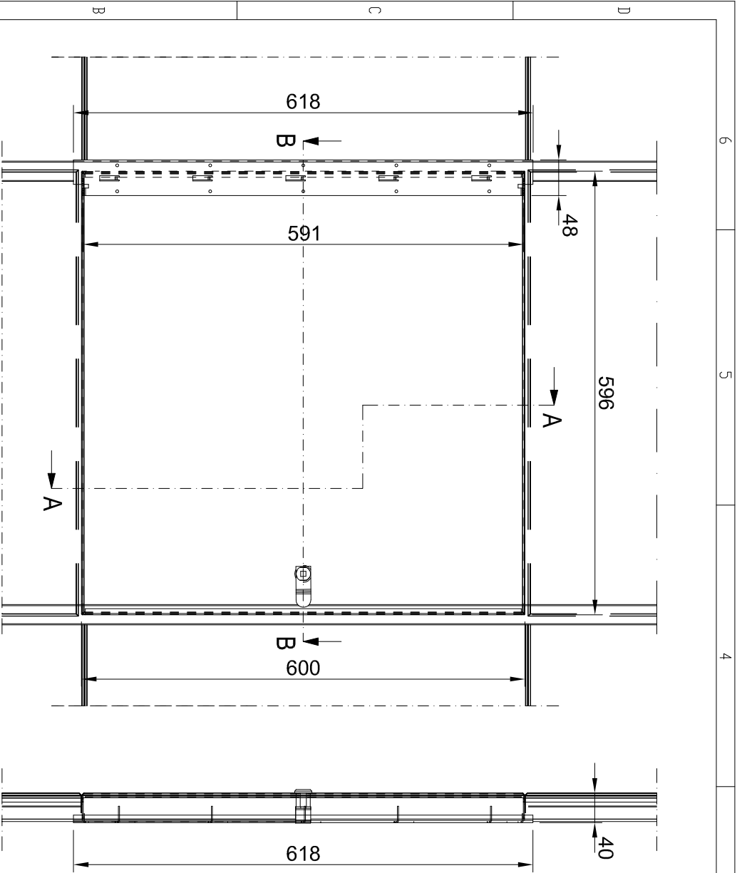
PLAN scale 1:5
